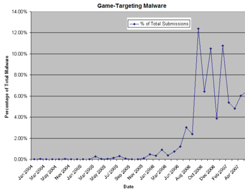
Figure 1: Malware growth in the last three years
